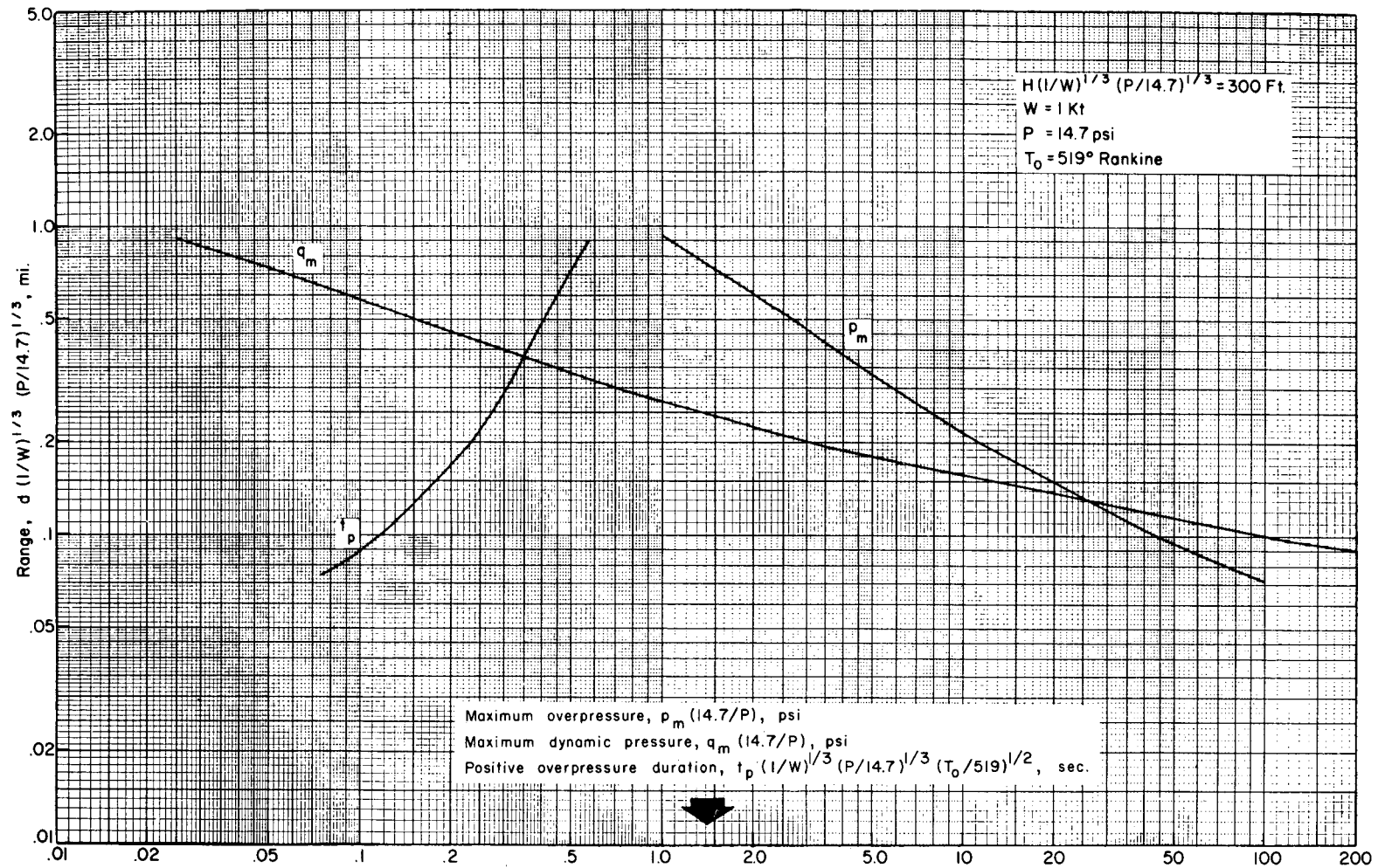
Fig. 2.4—Scaled blast parameters for a scaled height of burst of 300 ft as a function of scaled range. These are plots of Eqs. 2.30, 2.32, and 2.34 given in Table 2.4.
